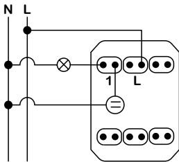
1 module - One-way switch with indication lamp
