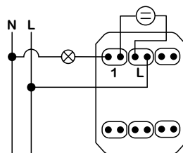
2 modules - Push-button with location lamp
