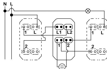
1 module - 2 two-way switches + 1 intermediate with location lamp
